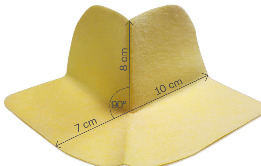
DRY CORNEROUT
