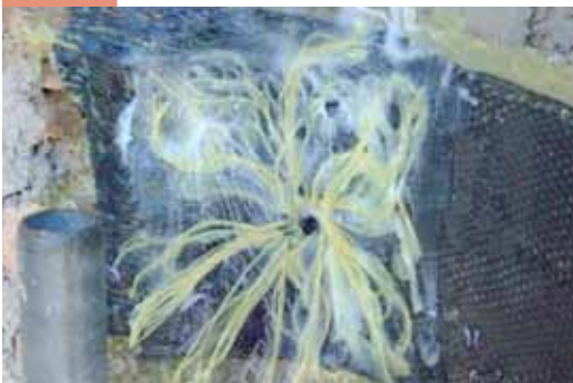
Fan-shaped opening of the thread and fixing with ARMOFIX MTX
