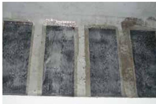
Application of ARMOSHIELD C-SHEET fabrics over the fresh coat of ARMOFIX MTX resin
