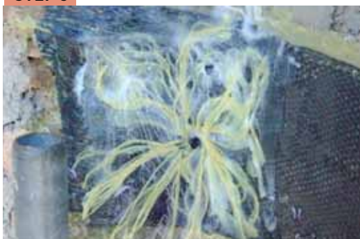
Fan-shaped opening of the thread and fixing with ARMOFIX MTX epoxy resin
