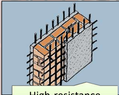
High-resistance structural plasters
